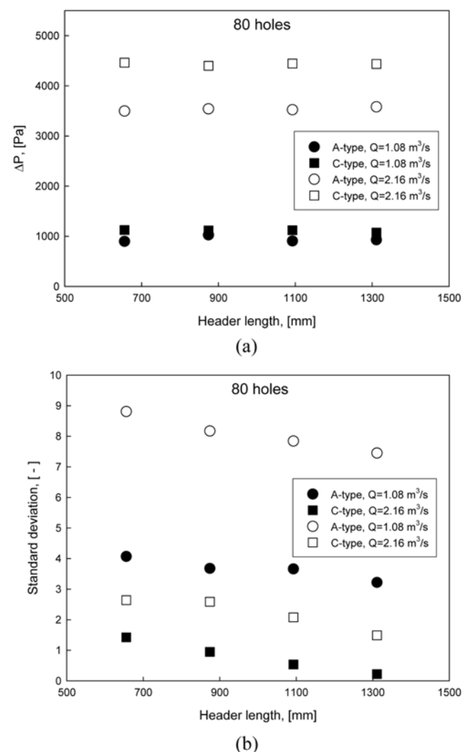
Fig. 7. Comparison of standard deviation and pressure drop for each header type according to the header length. (a) pressure drop, and (b) standard deviation.
